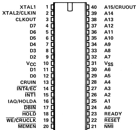
FIGURE 24 – PIN ASSIGNMENTS
