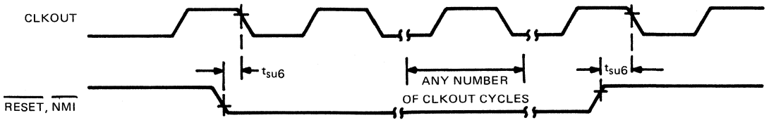
FIGURE 30 – TMS 9995 RESET AND NMI TIMING
