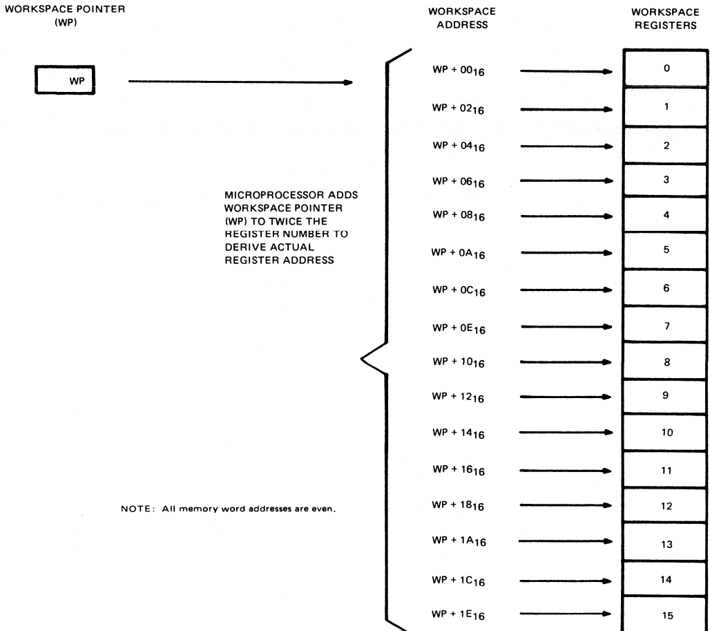
FIGURE 7 – WORKSPACE POINTER AND REGISTERS
