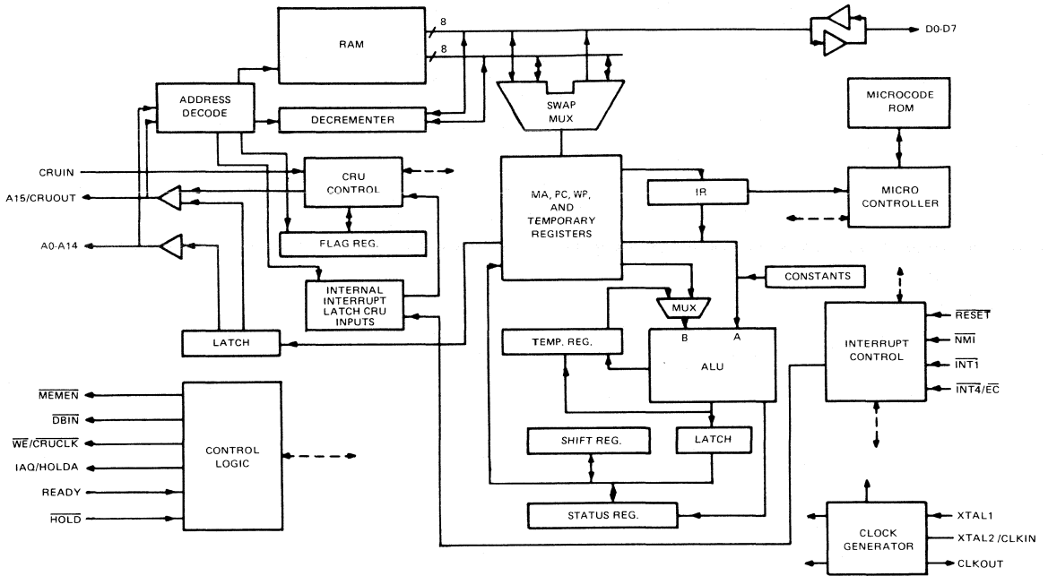
FIGURE 3 – TMS9995 BLOCK DIAGRAM
