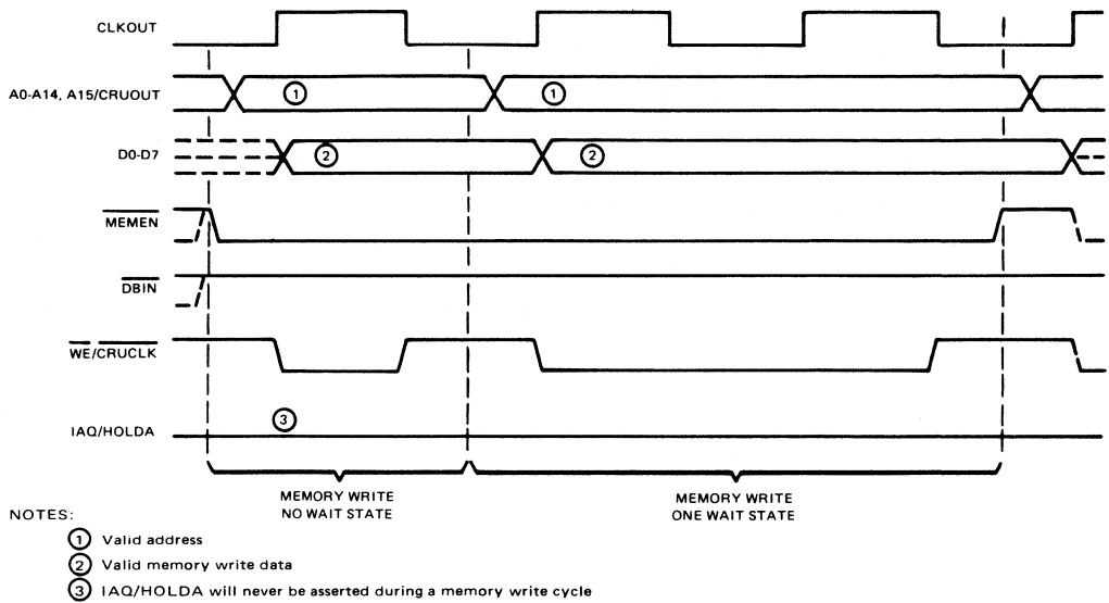
FIGURE 10 – TMS9995 MEMORY WRITE CYCLE
