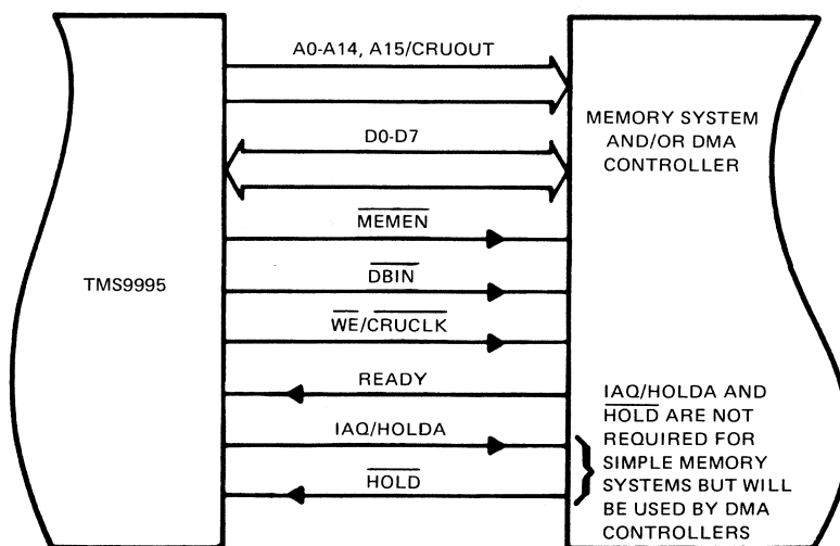
FIGURE 8 – TMS9995 MEMORY INTERFACE
