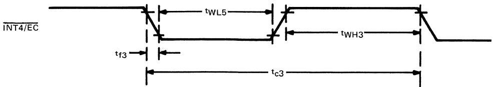
FIGURE 32 – TMS 9995 INTERRUPT INPUT TIMING
