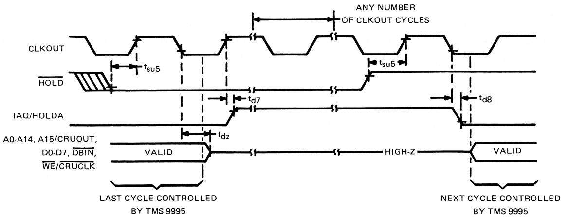
FIGURE 31 – TMS 9995 HOLD TIMING
