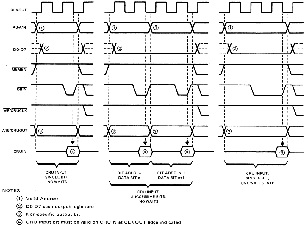
FIGURE 20 – TMS9995 CRU INPUT CYCLE
