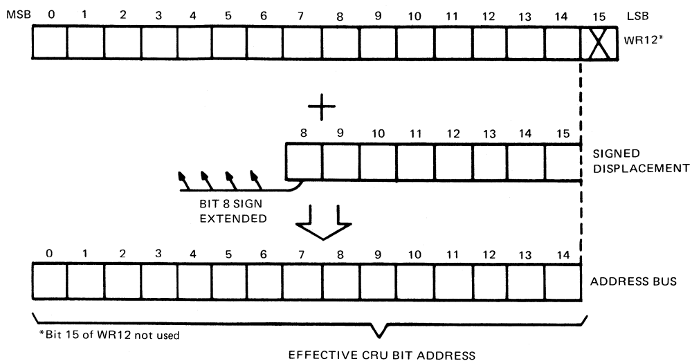
FIGURE 22 – SINGLE BIT CRU ADDRESS DEVELOPMENT
