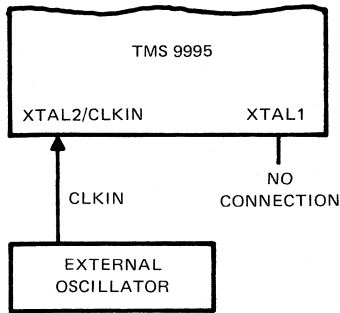
FIGURE 26 – EXTERNAL OSCILLATOR
