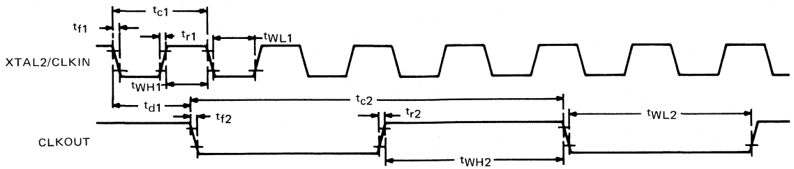
FIGURE 27 – TMS 9995 CLOCK TIMING
