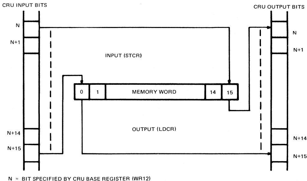
FIGURE 23 – LDCR/STCR DATA TRANSFERS
