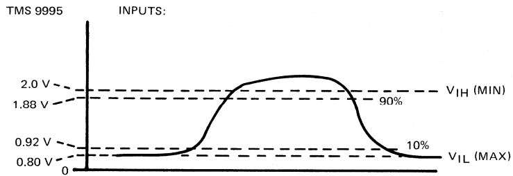
FIGURE 34 – MEASUREMENT POINTS FOR SWITCHING CHARACTERISTICS
