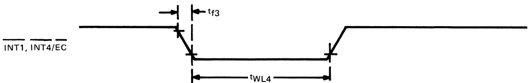
FIGURE 32 – TMS 9995 INTERRUPT INPUT TIMING
