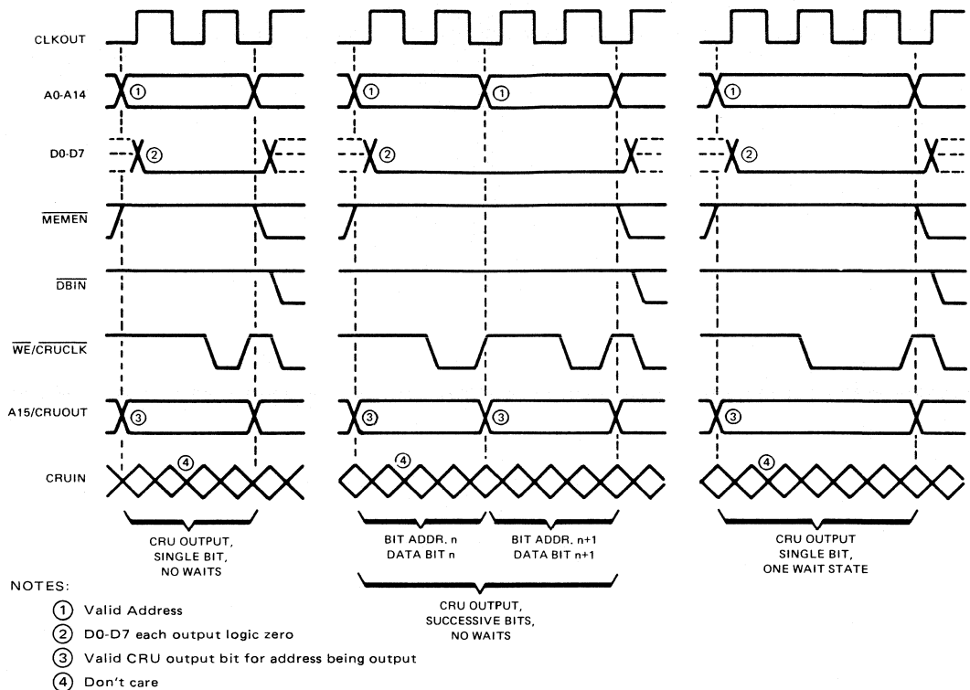
FIGURE 21 – TMS9995 CRU OUTPUT CYCLE
