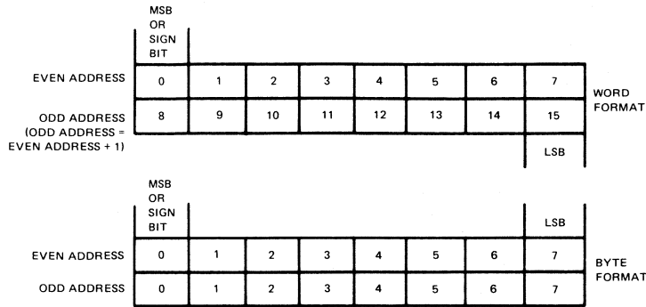
FIGURE 1 – WORD AND BYTE FORMATS
